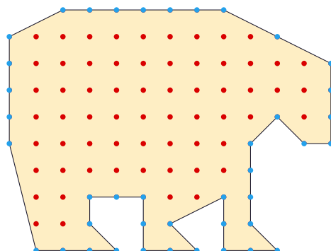
Figure 12: Ours – \bullet = 41 , \bullet = 63 , \square = 82,5
